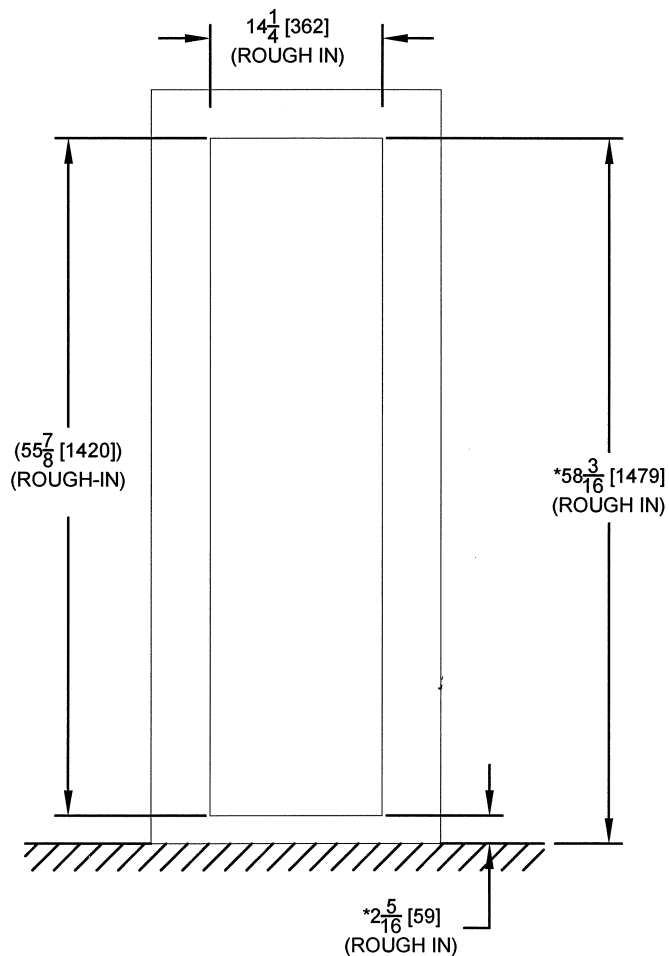
ROUGH-IN VIEW
