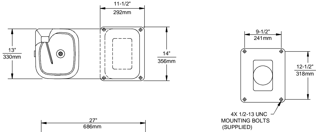
MOUNTING DETAIL
